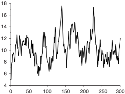
Autoregressive process (AR(1))
